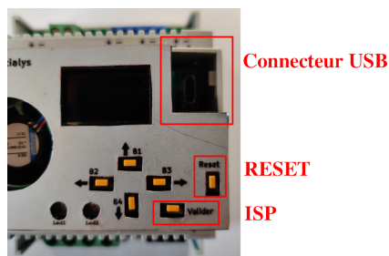
FIG 31 – Mode ISP
