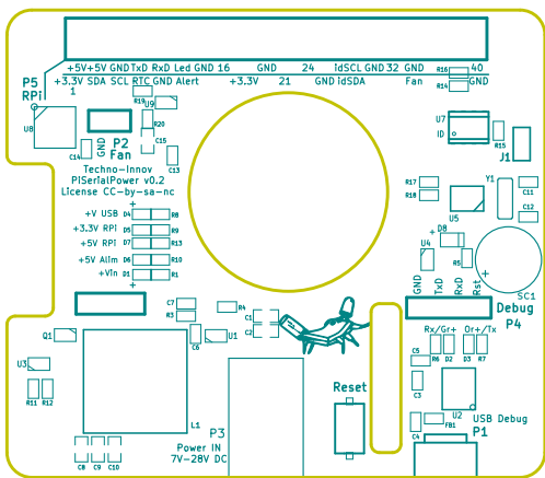
Top silk screen
