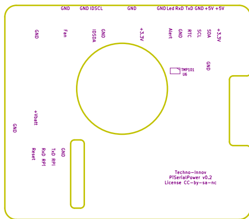
Bottom silk screen
